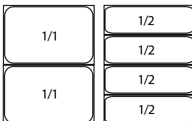
9F02 Prep Cart Dual End Loader Opening: 13" (33cm) Accommodates: 2 Rows
